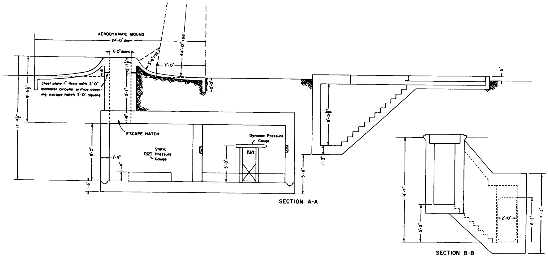
Fig. 2—Section of underground shelter 8001.
